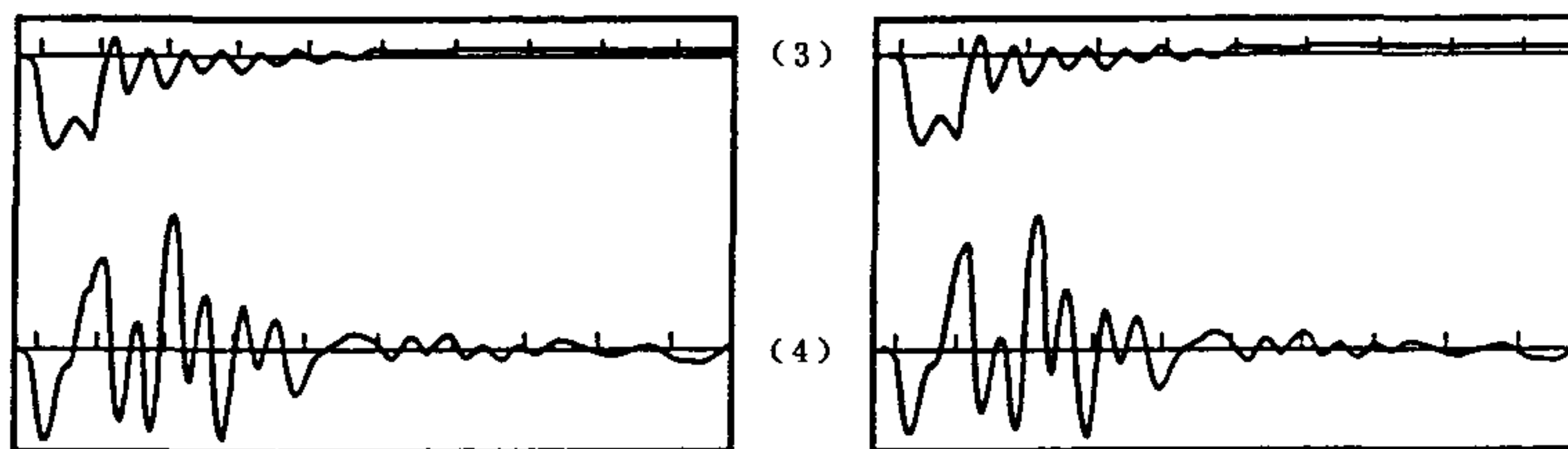
c) 降低电压截波 (62.5%)
